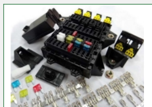
FUSE BOX- MVTYFB(20P)
